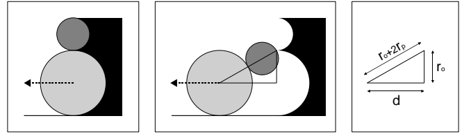
Fig. 11. Calculating the minimum distance d that O has to move to guarantee that \text{PR}_b(\tau(i_s + d)) \in \text{RVPR}(\tau(i_s + d), \sigma(i_s + d)) . The black area is the union of all possible obstacles. (a) The start of the object path section. (b) The first chance for P to reach \text{PR}_b(\tau(i_s + d)) . (c) The calculation of d . It is easy to see that d = \sqrt{4r_p^2 + 4r_p r_o} .
