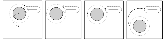
Fig. 8. An example of a pusher path that pushes O around a vertex. P is shown as a dot that represents its center. (a) The situation at the start of the section. The dotted arrow shows the trajectory of O . (b) First we push perpendicular to the compliant edge until an obstacle is encountered. (c) We follow the union boundary of the obstacles until \sigma(s) = \text{PR}_b(\tau(s)) . (d) Now we push following a circular shaped path having radius \sqrt{r_p^2 + 2r_p r_o + 2r_o^2} .
