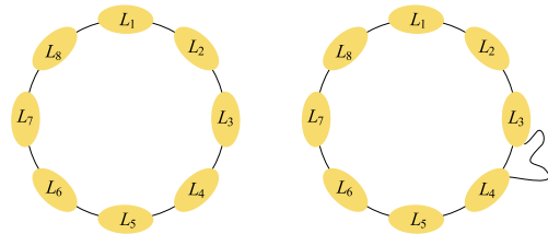
(a) A closed chain of labeled components each neighboring only two other labeled components. (b) The connection set CS(L_3, L_4, G) is extended.
